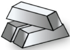
Mineral Ore
